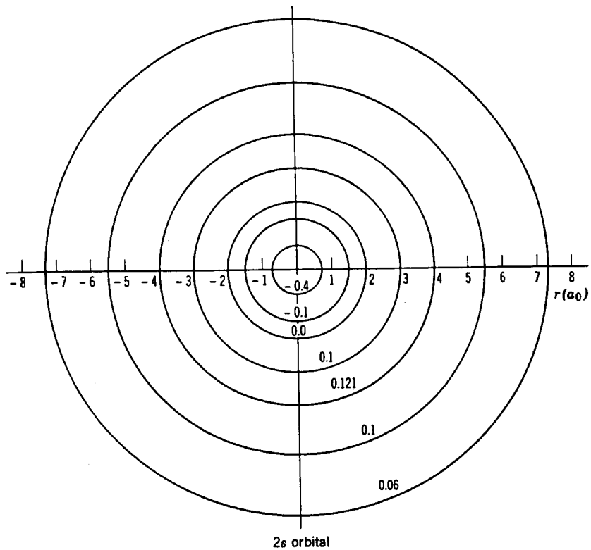
Fig. 1-10. Shapes of some atomic orbitals and hybrid orbitals. The numbers on the contours give the value of \psi .
